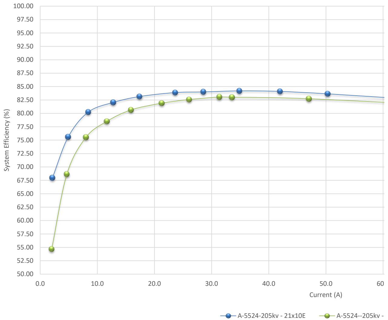
System Efficiency VS Current
