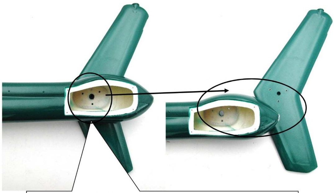
Align the tail fin 【35】 center hole, and adjust the angle, then drill three holes for mounting the fin through.
