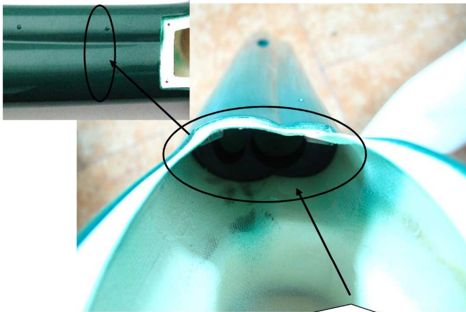
Slide the EVA dampener 【52】 through the tail rotor hatch into the tail boom, move it into the shown position.
