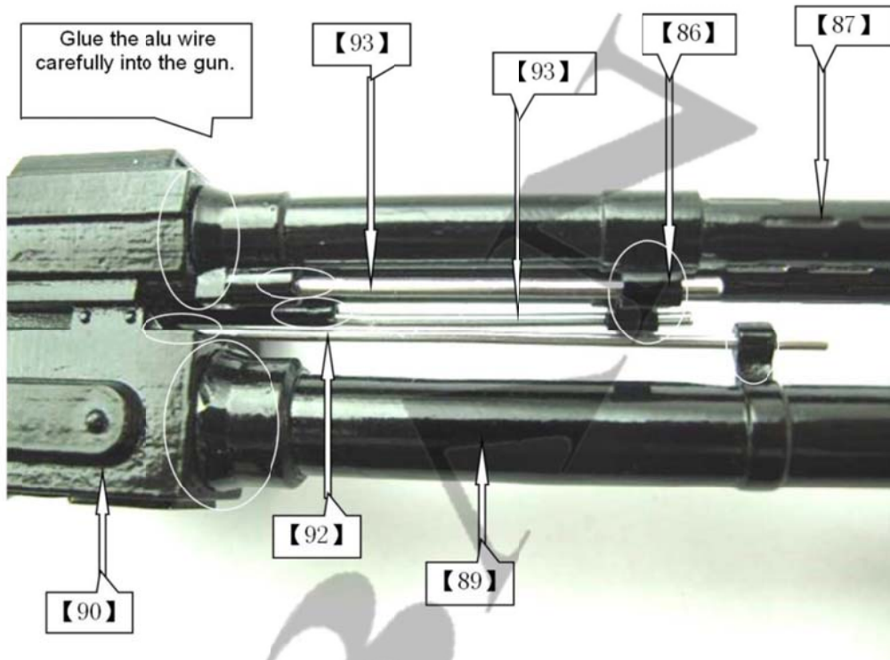
Completely assembled gun.
